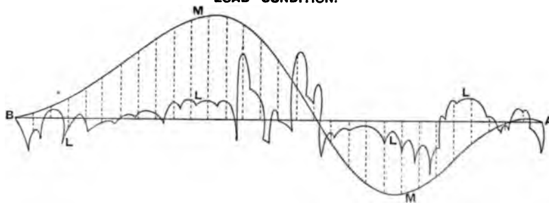
FIG. 112. LOAD CONDITION.
